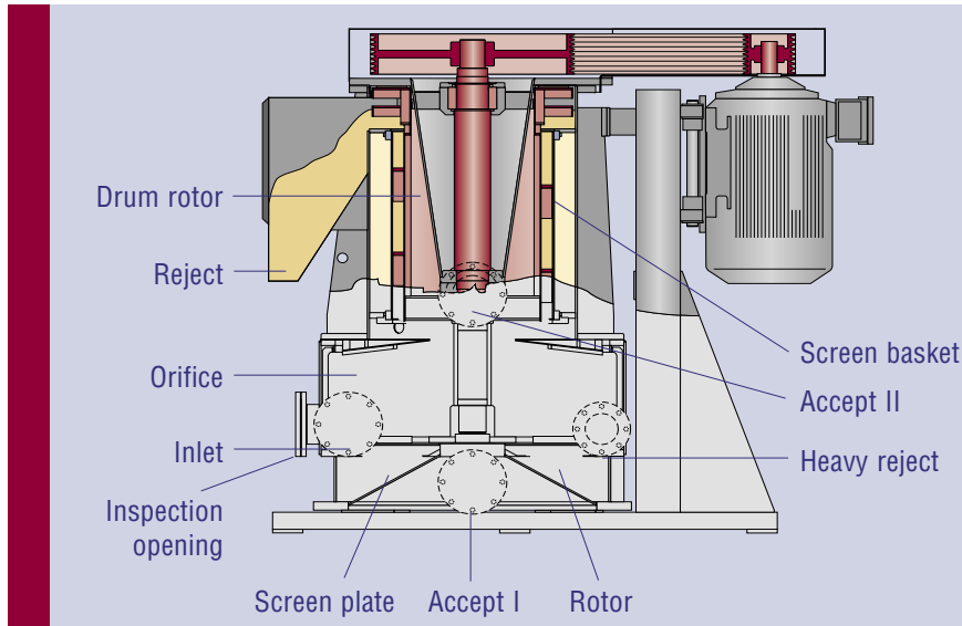
Combisorter™ CSM upper housing assembly major components
