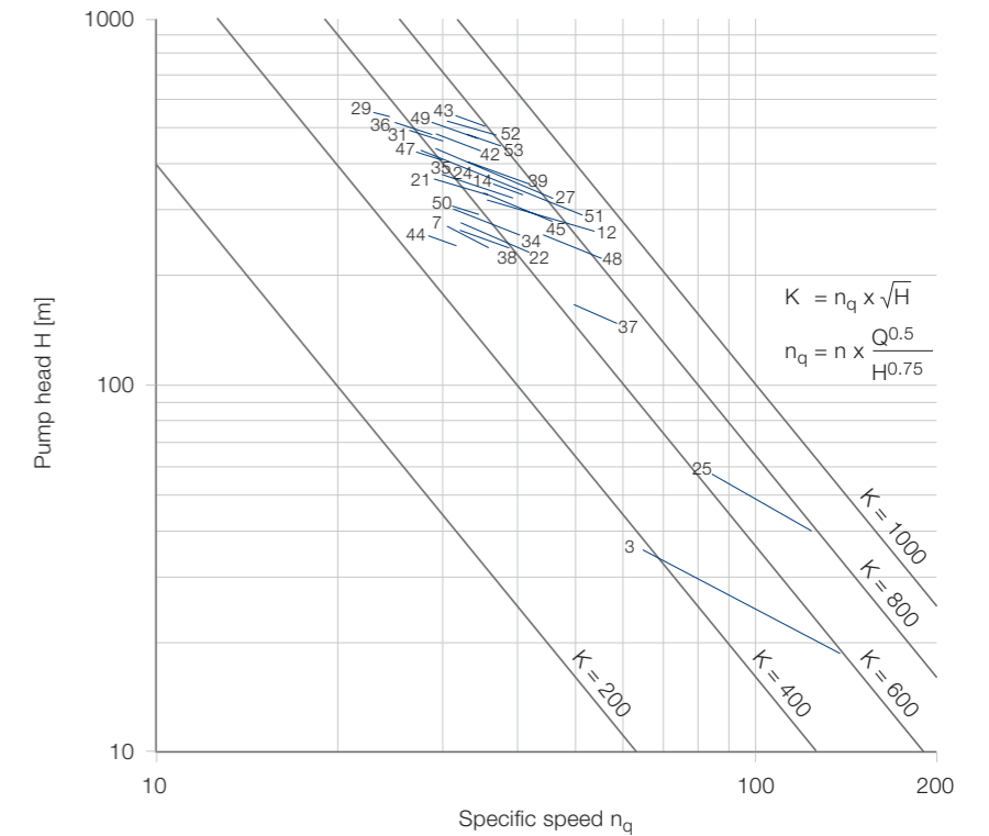
Selected pump-turbines: operation range in pump mode
